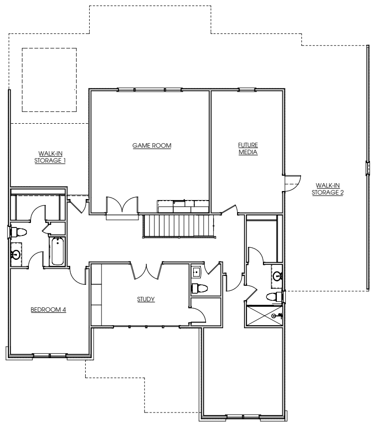
SECOND FLOOR
